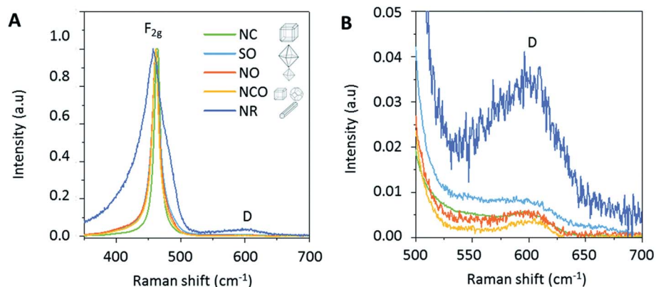
Fig. 5 (A) Raman spectra of CeO 2 particles recorded in between 350 and 700 \text{cm}^{-1} , and (B) between 500 and 700 \text{cm}^{-1} , where excitation source is at 633 nm. Reprinted from ref. 77 with permission © Royal Society of Chemistry 2020.
